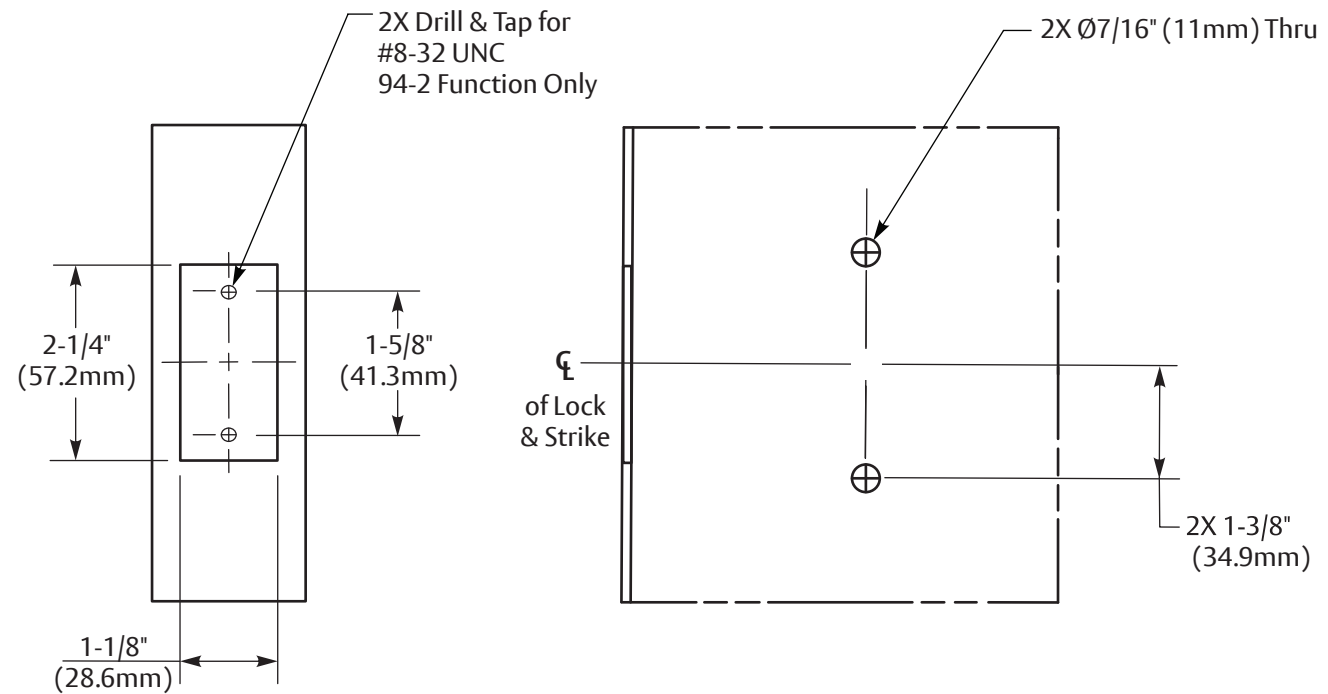
93/94 Functions Door Preparation
