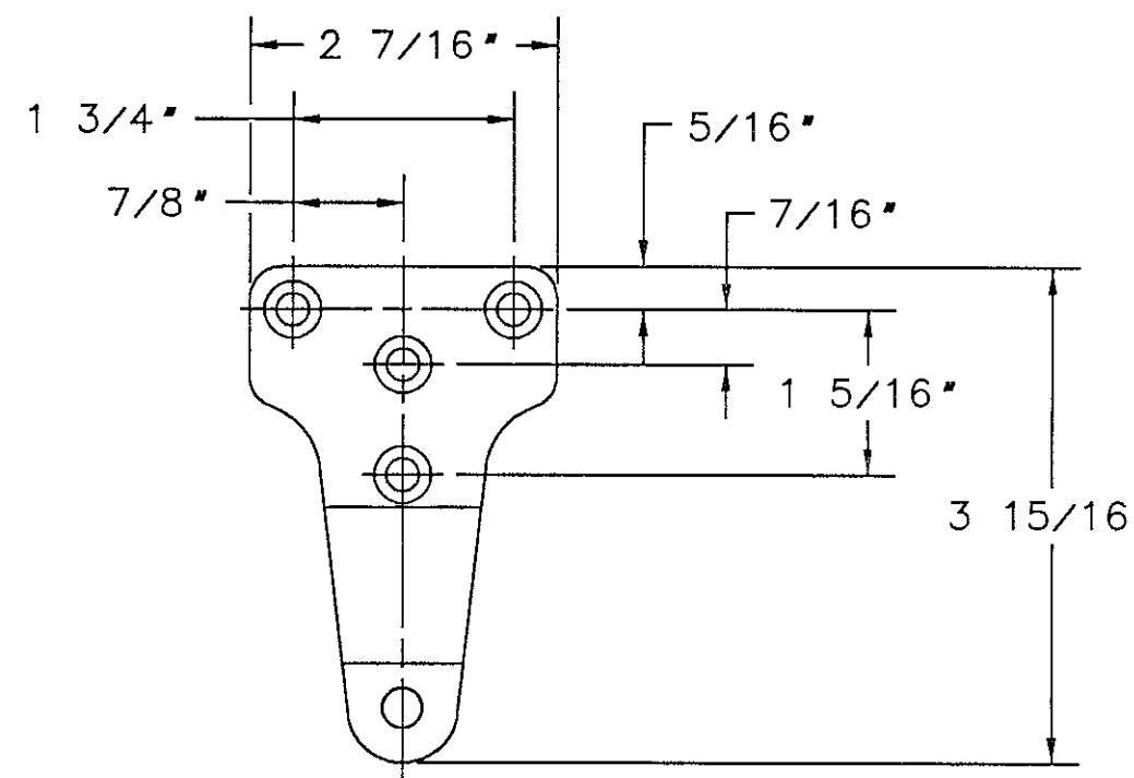
P3 BRACKET DETAIL
