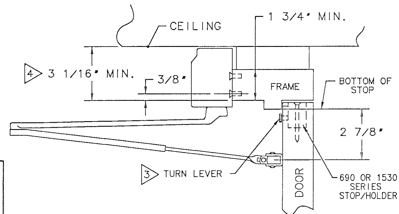
DOUBLE RABBETED FRAME (690 SHOWN)
