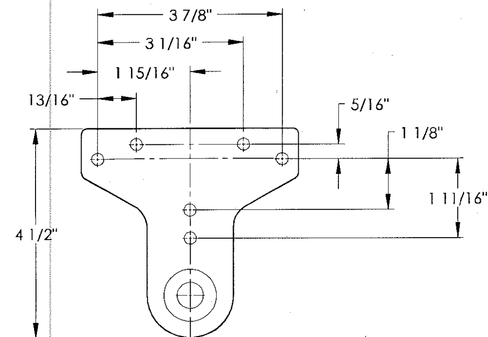
P10 FOOT BRACKET DETAIL
