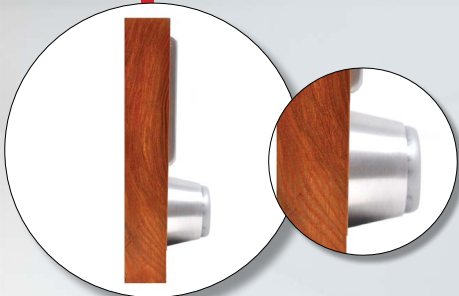
Sloped Door Armature Assembly without Extension Plates - 1-1/2" Projection
