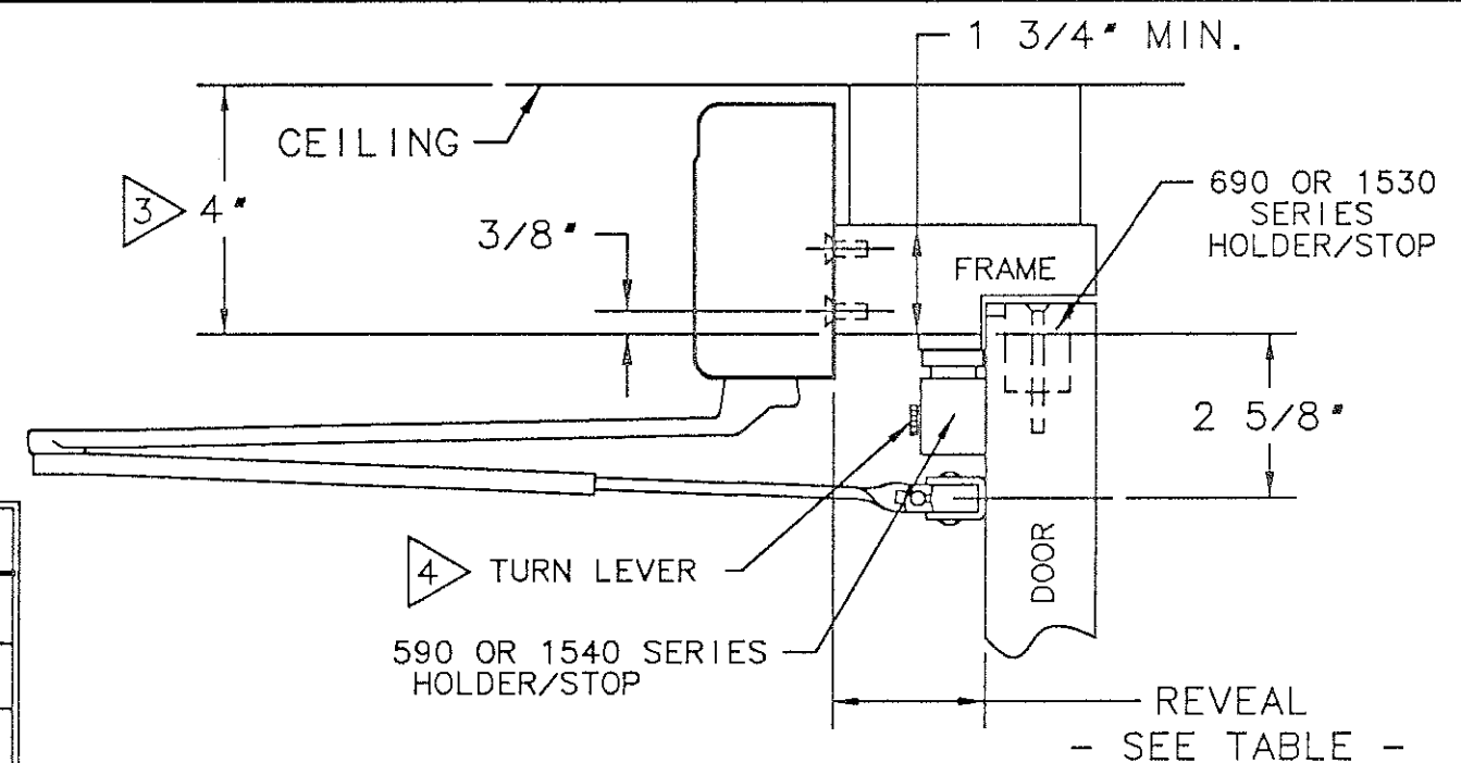
SINGLE RABBETED FRAME (590 & 690 SHOWN)
