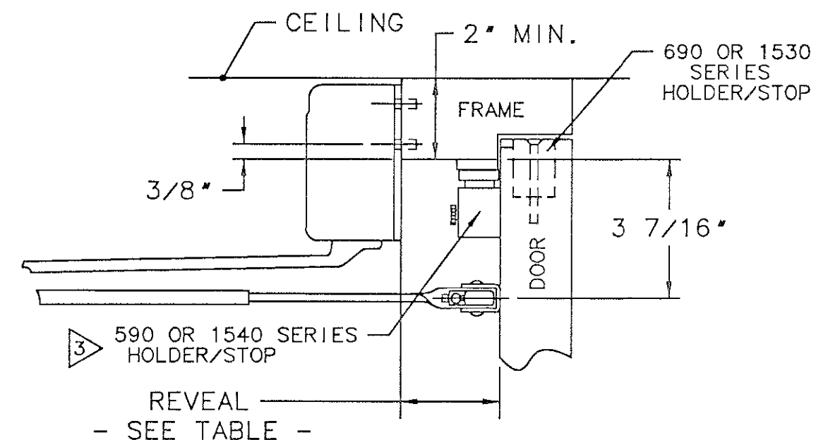
SINGLE RABBETED FRAME (590 & 690 SHOWN)
