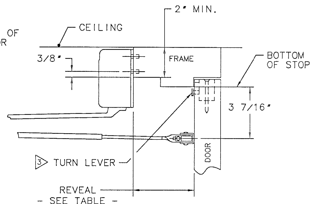
DOUBLE RABBETED FRAME (690 SHOWN)
