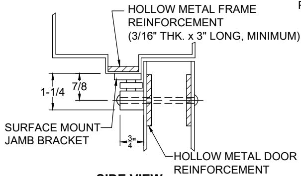
SIDE VIEW CROSS SECTION
