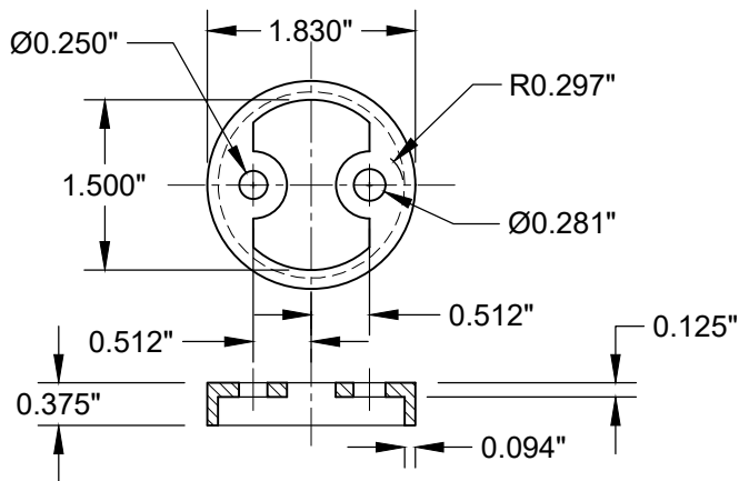
RM444 - RISER BASE
