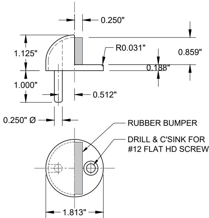
RM441 - DOME STOP BASE
