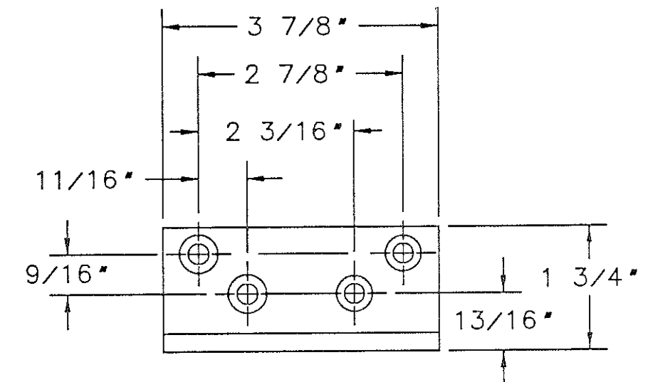
195 ANGLE BRACKET DETAIL
