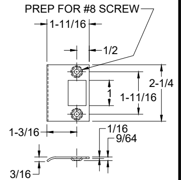
WOOD FRAME ("T" STRIKE SHOWN FOR EXAMPLE)
