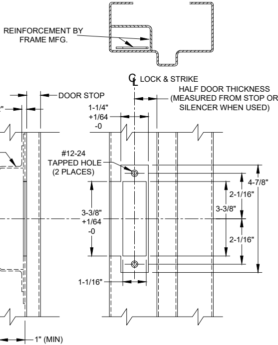
METAL FRAME (ASA STRIKE SHOWN FOR EXAMPLE)
