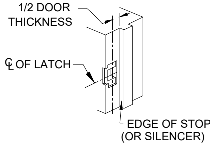
WOOD FRAME ("T" STRIKE SHOWN FOR EXAMPLE)
