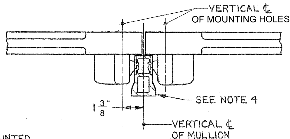
DOUBLE DOOR WITH 650 A MULLION (1 3/4" MIN. STILE)
