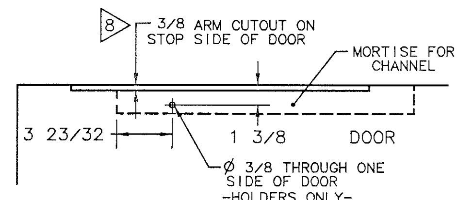
SECTIONAL VIEW WITH DOOR CLOSED
