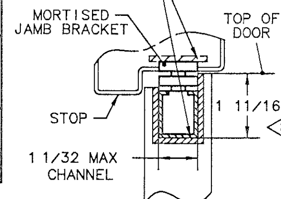
SECTIONAL VIEW WITH DOOR CLOSED
