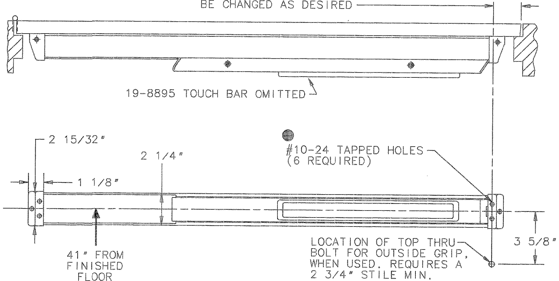
8895 EXIT DEVICE ILLUSTRATED
