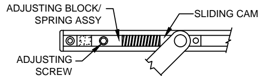
SINGLE ACTING DOOR
