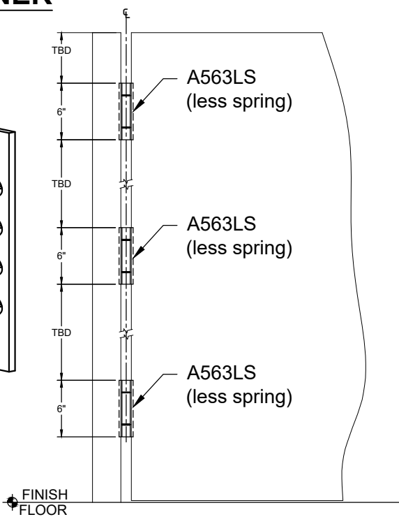
Front view of Door Hinge Location for example
