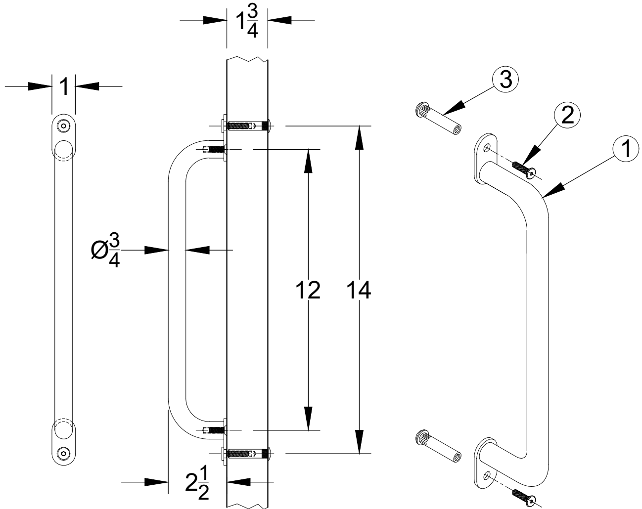
PULL HANDLE
