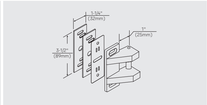
793 Optional strike for double door applications without a mullion. Supplied with #10-24 x 3/4" machine screws, two shims (each 1/16" thick), and one locking plate.
