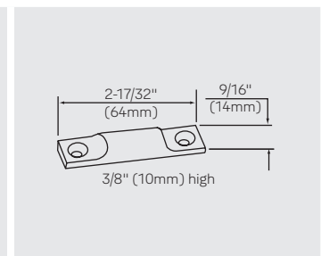
702 Optional bottom strike for bottom pullman latch option. Supplied with #8 x 8/32" combination screws.
