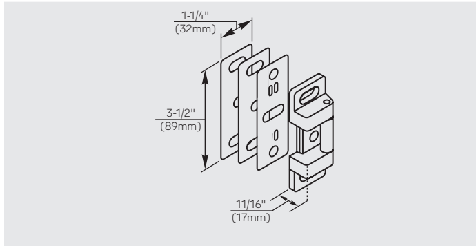
757F Standard strike for 1800(F) devices. Supplied with #10-24 x 3/4" machine screws, two shims (each 1/16" thick), and one locking plate.
