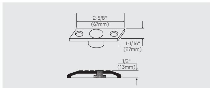
794 Optional bottom strike for fire openings using saddle thresholds or for flush floor mount. Must use for fire openings with 1/2" thresholds. Supplied with #10-24 x 1/2" machine screws and floor anchors.
