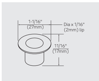
790 Standard bottom strike for 7110(F), 7120(F), 7160(F), 7170(F), 7210, 7220, 7210M(F), 7220M(F) series devices. Press in place.
