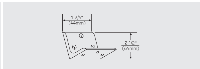
797 Optional bracket for mounting 791 top strike in flush transom opening. Supplied with 1/4-20 machine screws; SN-134 sex nuts, optional.
