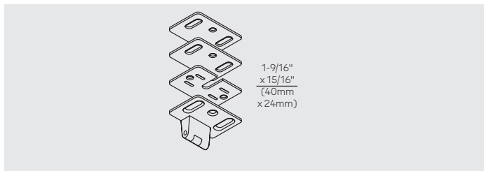
791 Standard top strike for 1810(F) devices. Supplied with #10-24 x 3/4" machine screws, two shims (each 1/16" thick), and one locking plate.
