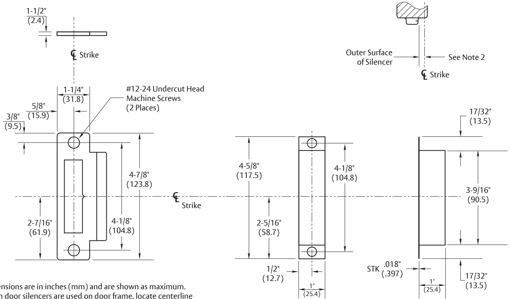
Detail of Strike Box
