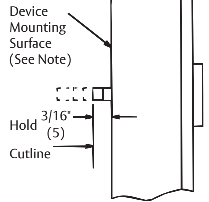
Figure 1. Device Mounting Surface (See Note)
