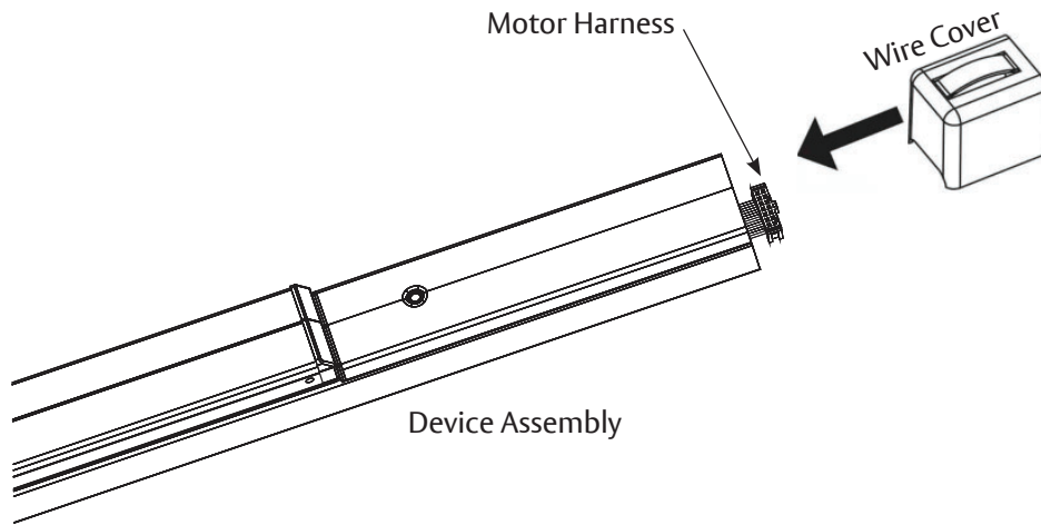
Figure 2: Installing Wire Cover
