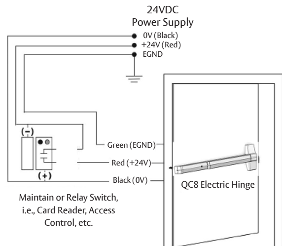
Figure 14: MELR 7000 Series Exit Device Typical Power Mode Wiring
