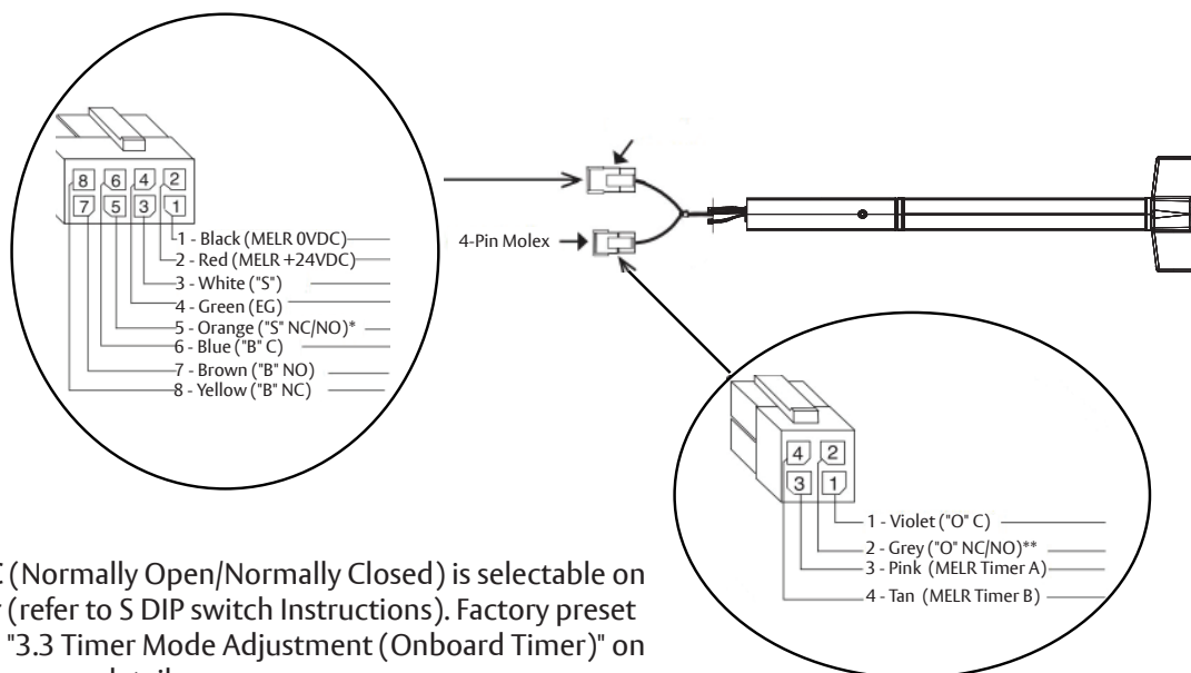
Figure 5: Wire Color and Position
