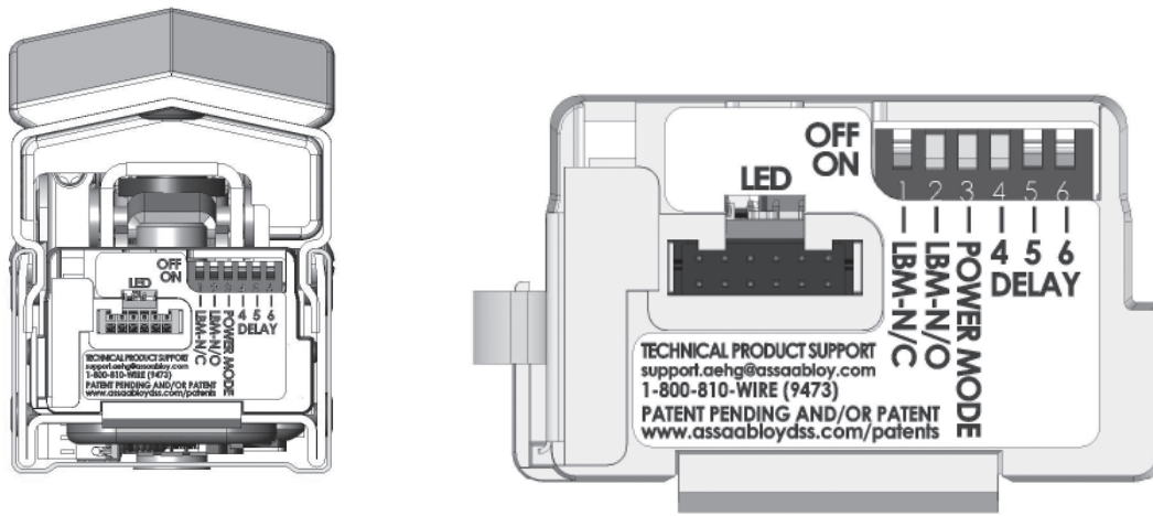
Figure 6: DIP Switch Settings (Factory Default Shown)
