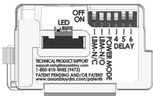
Figure 12: DIP Switch Setting for Power Mode Installation
