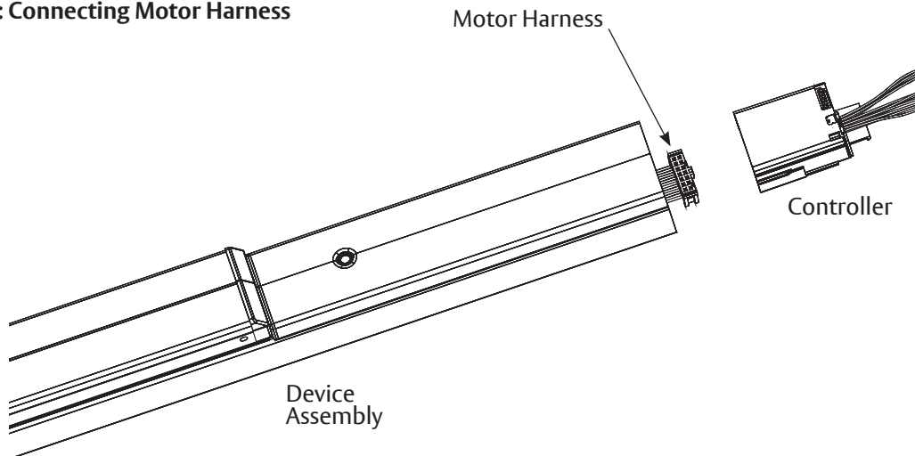
Figure 3: Connecting Motor Harness
