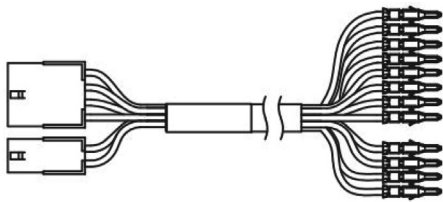
Figure 13: Molex with 12-Pin Connector Pinned
