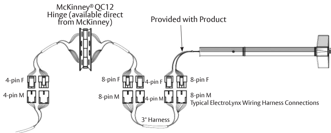
Figure 8: Typical ElectroLynx Wiring
