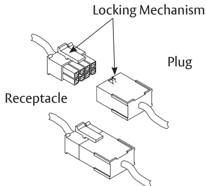
Figure 8: Typical ElectroLynx Wiring
