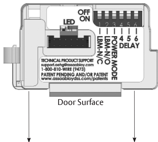
Figure 16: DIP Switch Setting for Timer Mode Installation
