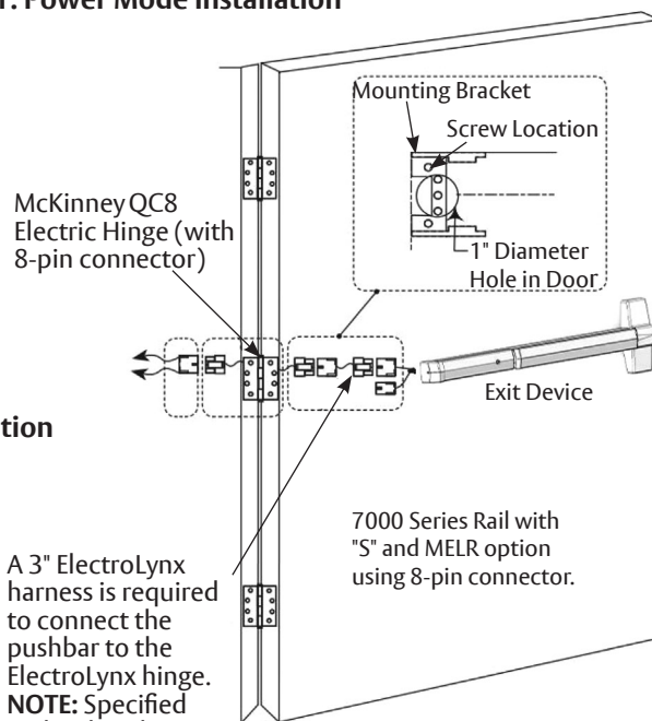
Figure 11: Power Mode Installation
