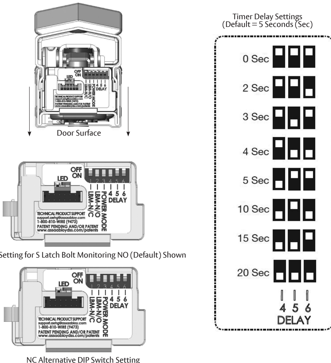
Figure 21: DIP Switch Settings
