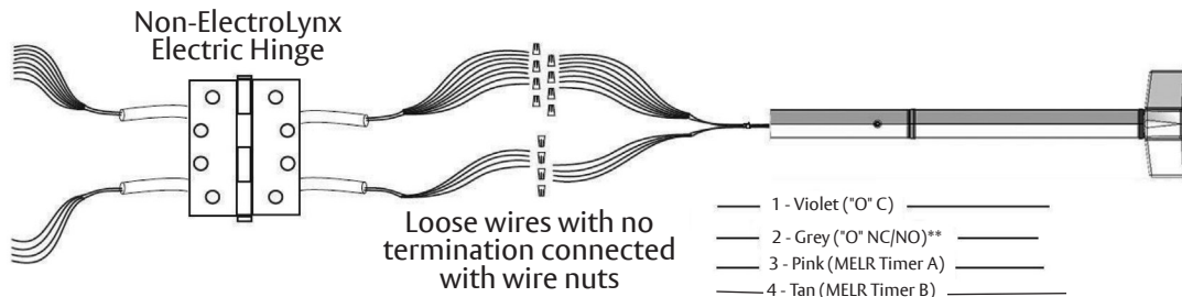
Figure 19: Timer Mode Typical Wiring
