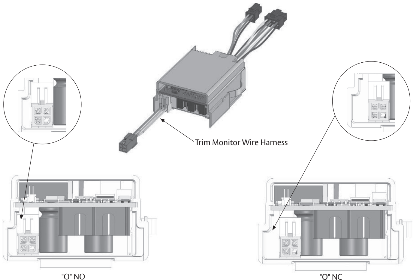
Figure 22: Changing O Preset
