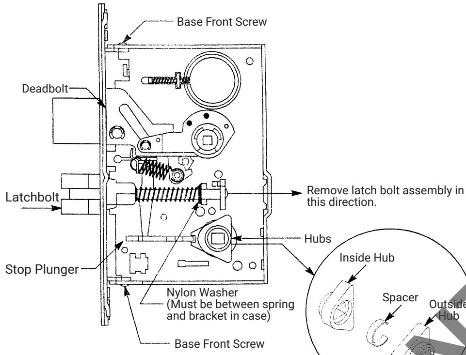
Lock Body (cover removed) LHR Shown
