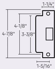
Model No. YR02030* ANSI 4-7/8 Strike
