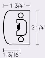
Model No. YR02001* Full Lip Strike Square Corner
