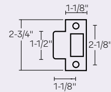
Model No. YR02020* T-Strike
