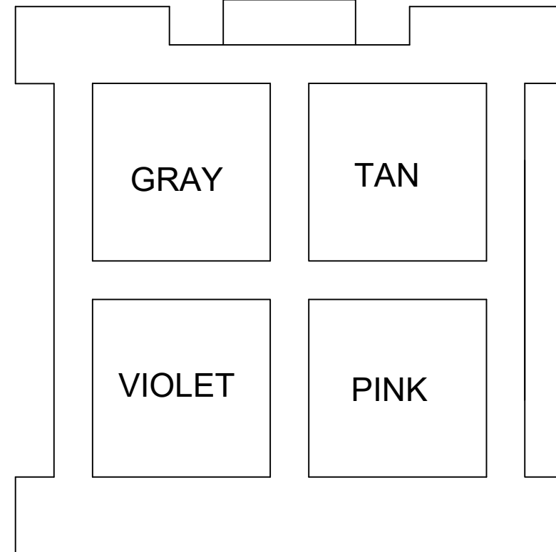
4 - MALE PIN HOUSING MOLEX CONNECTOR MICRO-FIT 3.0 (43020-0401) ABH-3301
