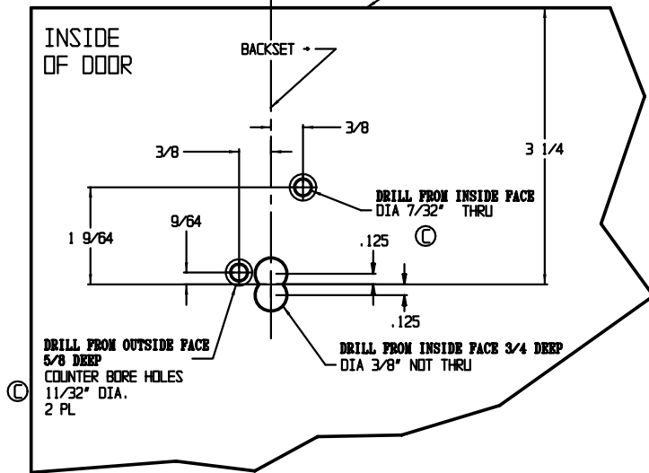
DETAIL -C-
