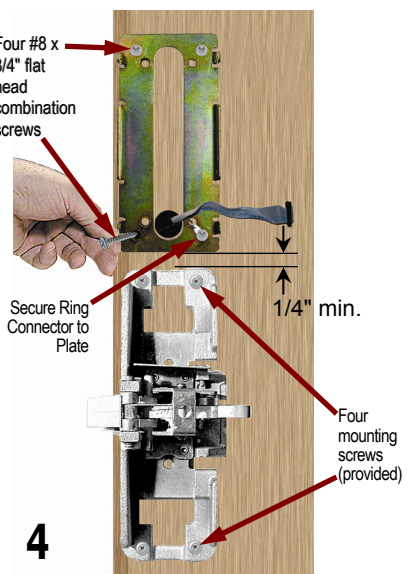
4. Replace Exit Device, insert and fasten with 4 new mounting screws (do not over-tighten). Before mounting the Battery Box Mounting Plate, carefully pull wires from door through center of Plate. Do not pinch or cut wires. Position the Plate a minimum of 1/4" above Exit Device. Fasten the Battery Box Mounting Plate with four #8 x 3/4" flat head combination screws, using one of the screws to secure the green ground wire ring connector to the Plate.
