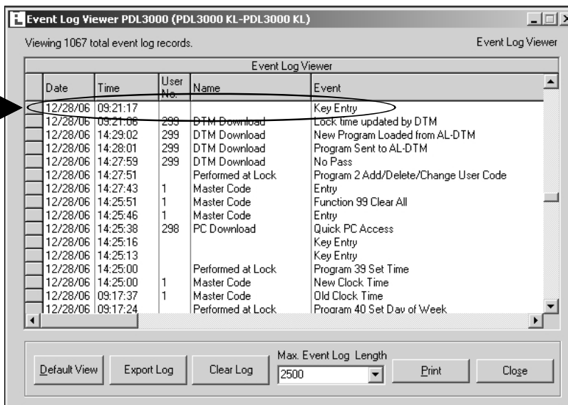
Sample log entry as displayed by DL-Windows (v3.6.0 or later).
