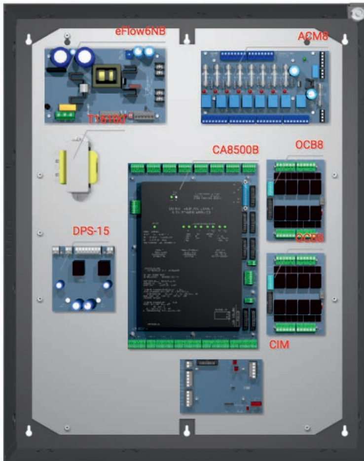
T2KK3F8 8-Door Access System with Power
