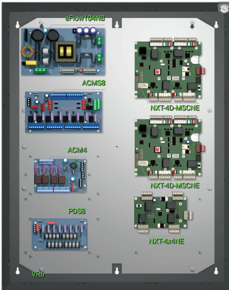
T2KSK7F12 12-Door Access System with Power
