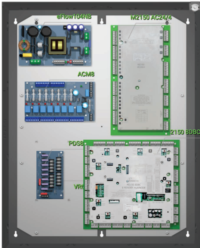
T2AMK7F8 8-Door Access System with Power
