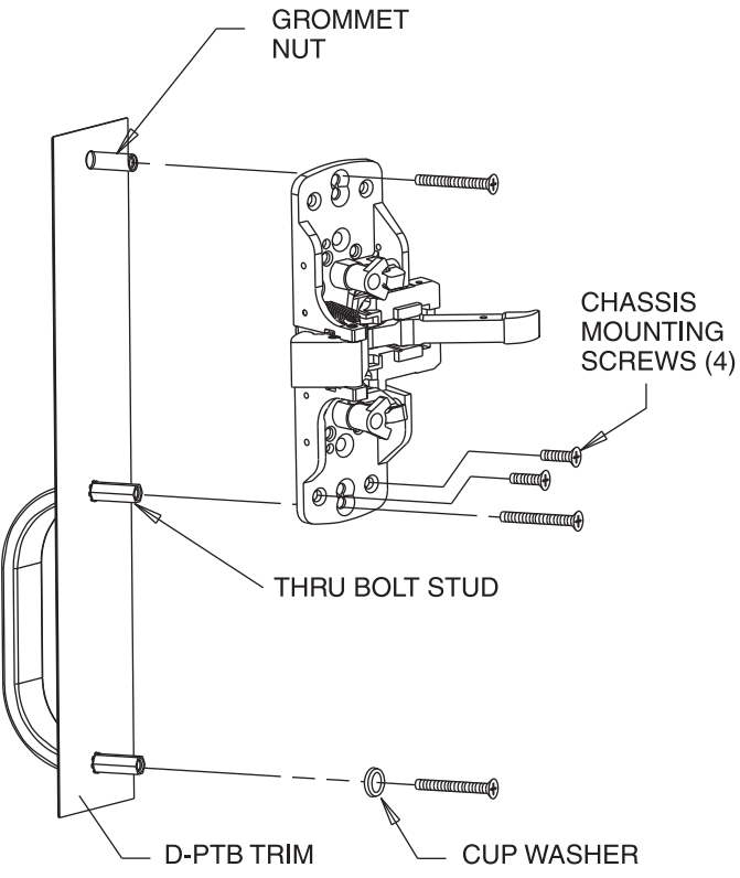
SINGLE DOOR MOUNTING ONLY
