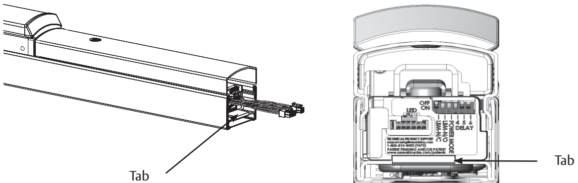
Figure 4 Tab attachment
