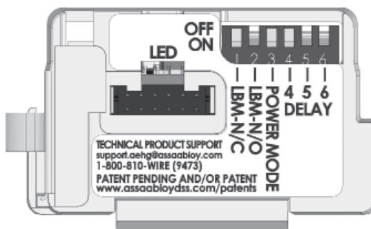
NC Alternative DIP Switch Setting
