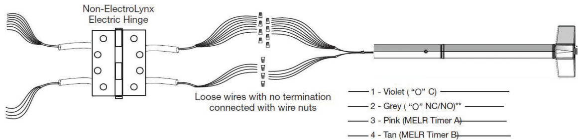
Figure 19 Timer Mode Typical Wiring
