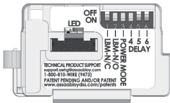
DIP Switch Setting for M91 Latch Bolt Monitoring NO (Default) Shown
