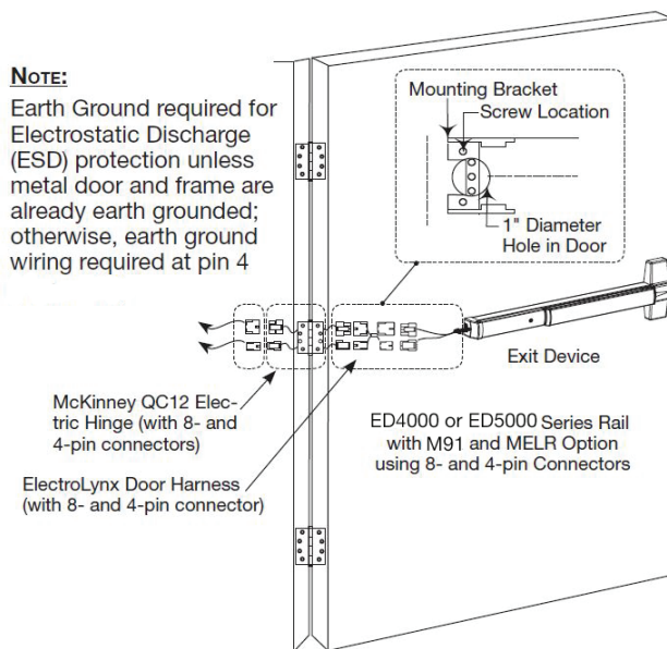
Figure 17 Timer Mode Installation
