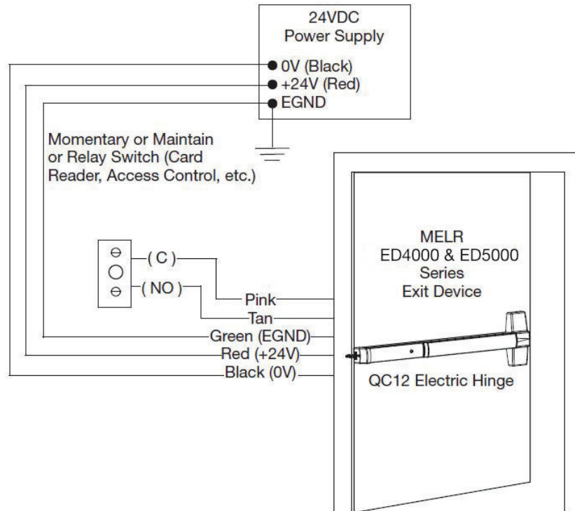
Figure 20 Non-ElectroLynx Timer Mode Connection MELR Wires with ElectroLynx Connector Removed
