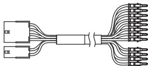
Figure 13 Molex with 12-Pin Connector Pinned
