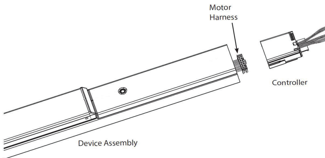
Figure 3 Connecting Motor Harness
