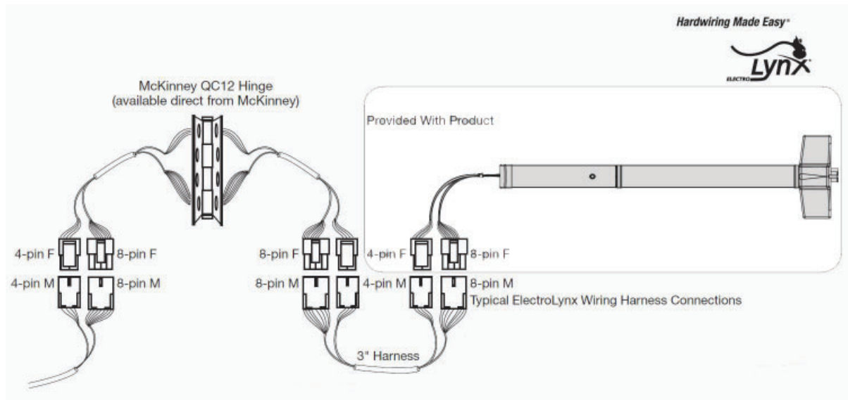
Figure 8 Typical ElectroLynx Wiring
