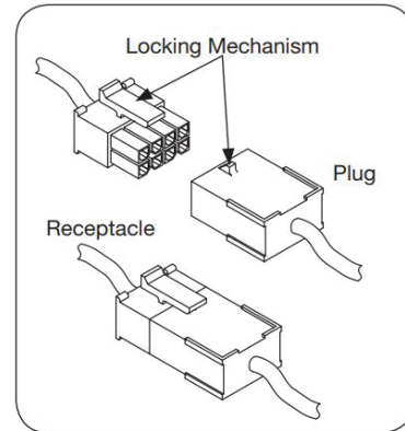
Figure 7 ElectroLynx Connections
