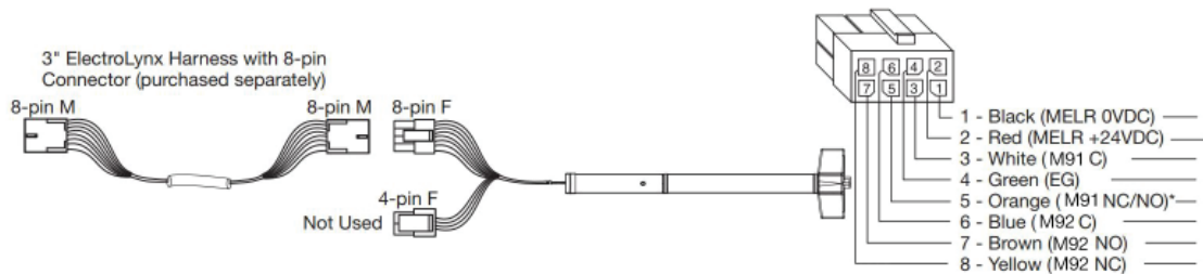
Figure 9 Typical ElectroLynx Power Mode Wiring
