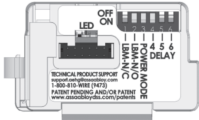
Figure 6 DIP Switch Settings (Factory Default Shown)
