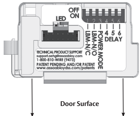
Figure 16 DIP Switch Setting for Timer Mode Installation
