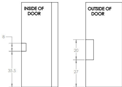
VERTICAL ROD DEVICE
