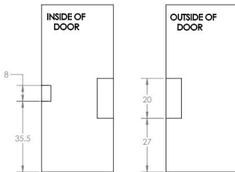
RIM DEVICE
