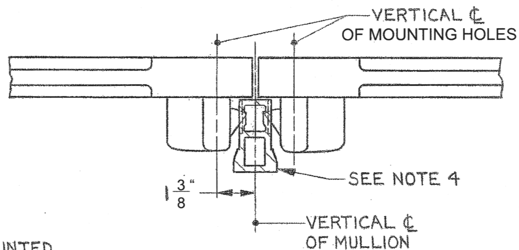
DOUBLE DOOR WITH 650 A MULLION (1 3/4" MIN. STILE)
