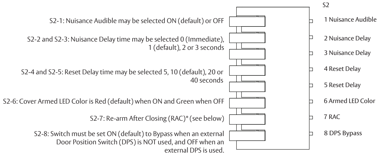
PCBA DIP SWITCH VIEW
