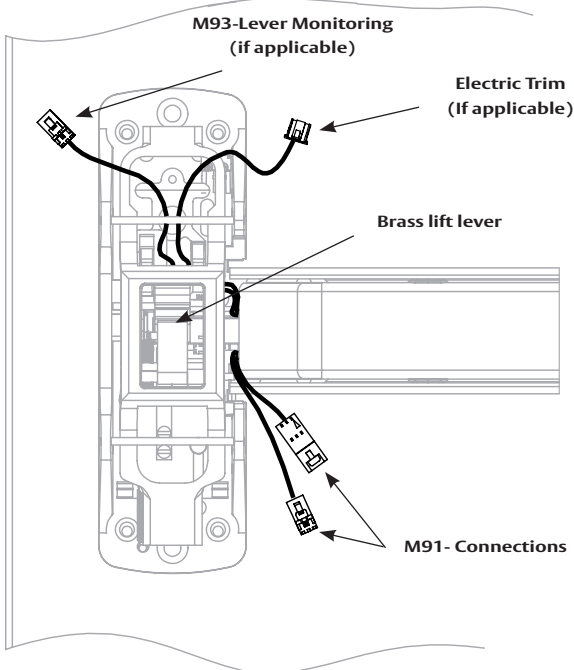
Step 1. Install chassis and rail (Section 4). Route trim wires from rail under brass lift lever as shown.
