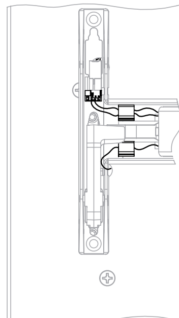
Step 5. Pull back excess wire through rail. Route wires as shown. Install wire clips.
