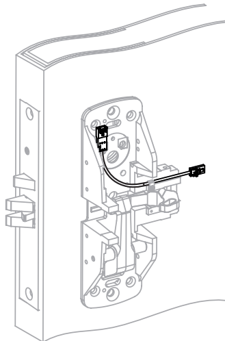
Step 2. Install chassis and connect M91 jumper at chassis.
