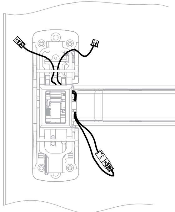
Step 2. Make M91- connection.
