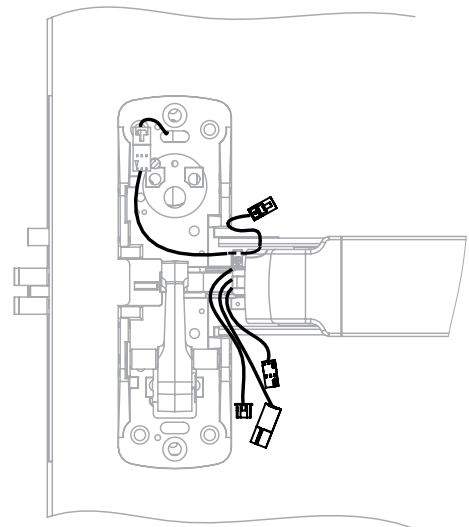
Step 3. Install rail to chassis.
