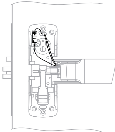
Step 6. Pull back excess wire through rail. Step 6. Pull back excess wire through rail.
