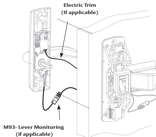
Step 4. Make trim wire connections and secure trim to door. Pull back excess wire through rail.
