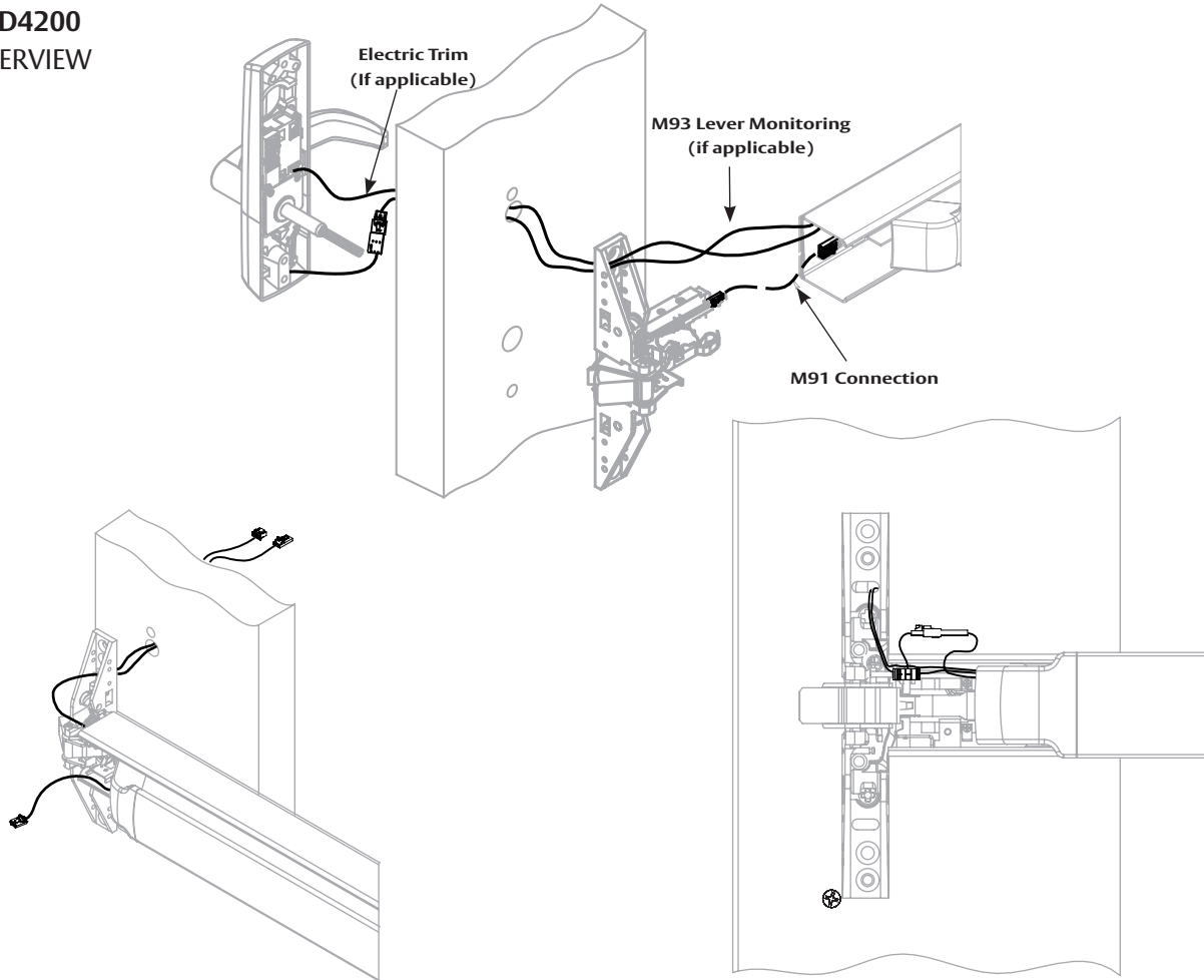
Step 1. Install chassis to rail. Route wires through door as shown.
