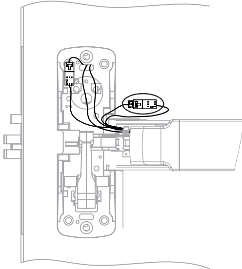
Step 4. Make wire connections.
