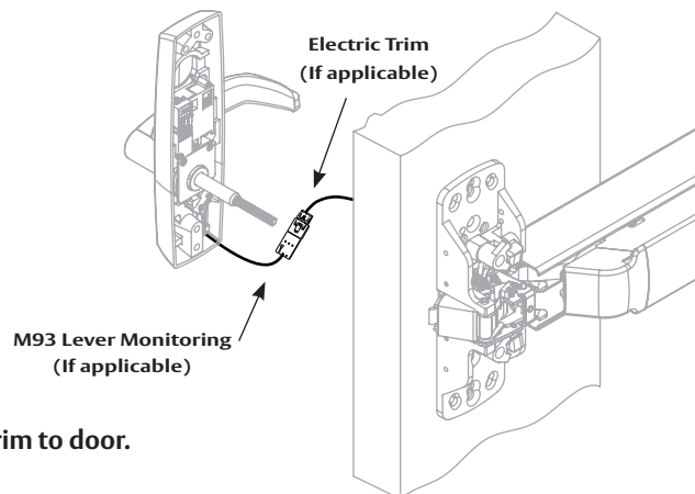
Step 2. Route trim wires through chassis and door as shown above.
