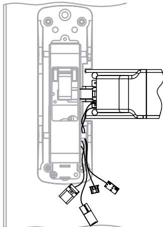
Step 3. Install rail.
