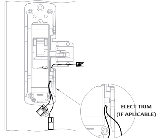
Step 2. Install chassis (Section 4) and route wires through chassis as shown.
