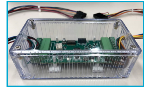
(SNT1) WTB OSDP adapter wiring harness
