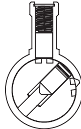
Cutaway cylinder showing construction master key being used, putting the wafer below the shear line while key is turned. Note the two empty "donut" holes on either side of the chamber.
