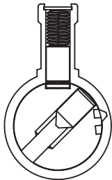
As change key rotates, construction wafer falls into "donut" hole in the side of plug. Only construction wafer will fall due to hole through its center. This voids the construction feature.
