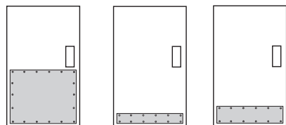
ARMOR PLATE ANSI J101 Metal J105 Plastic MOP PLATE ANSI J103 Metal J107 Plastic KICK PLATE ANSI J102 Metal J106 Plastic
