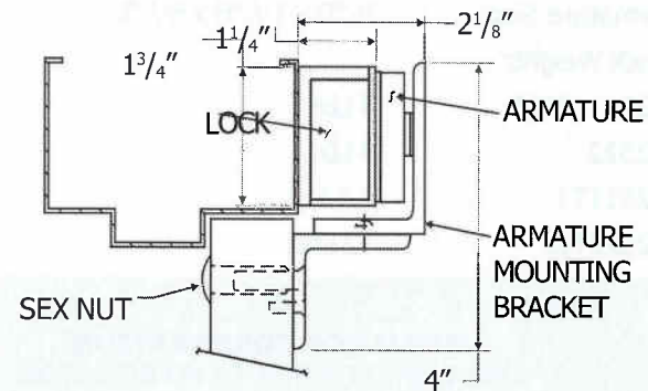
2511TJ SIDE VIEW
