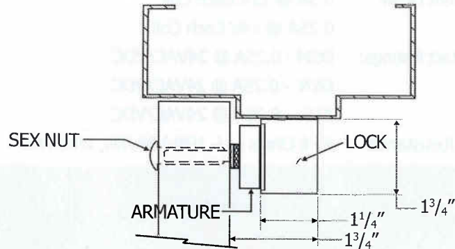
2511/2585 SIDE VIEW
