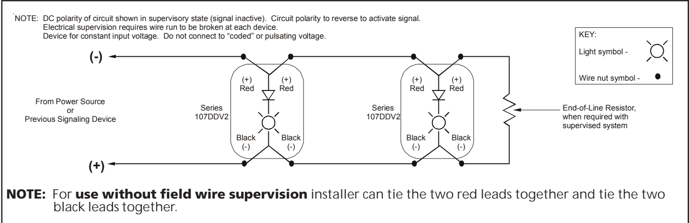
Figure 4. Wiring Diagram
