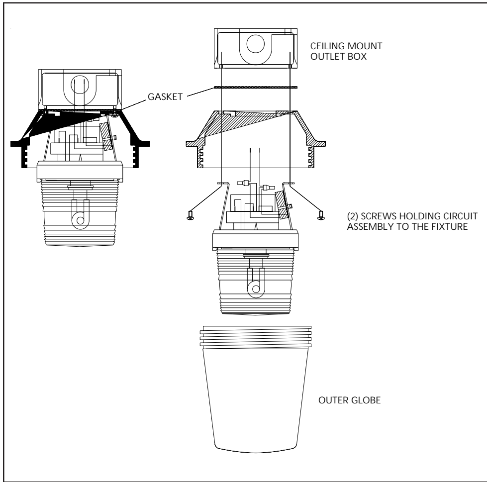
Figure 5. Disassembly of the 107DDV2 Series AdaptaBeacons
