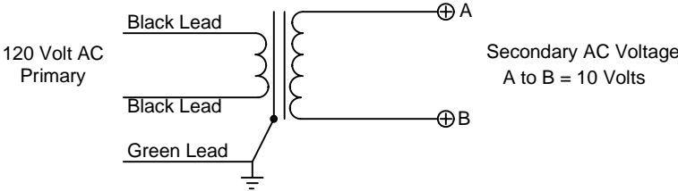
590 Transformer
