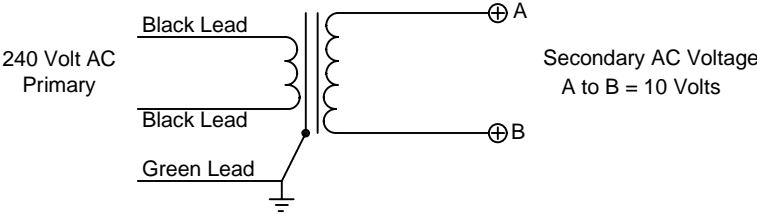
590Y Transformer
