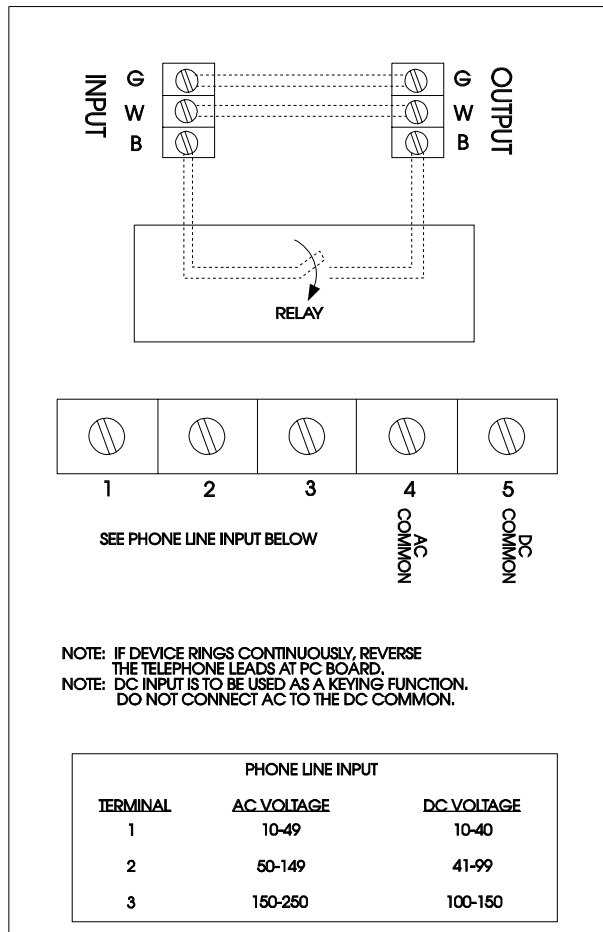
Figure 2. Electrical Connections (Screw terminals accept 26-12 AWG wire size)
