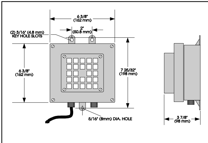
Figure 1. Phone Horn Dimensions
