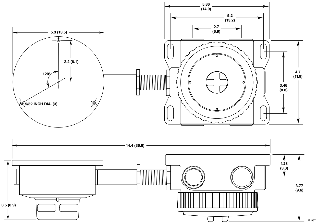
Figure 2—U5005 Dimensions in Inches (Centimeters)
