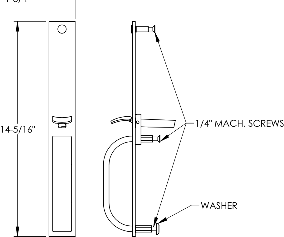
TRIM NO. 828 FLL DESIGN
