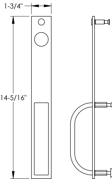
TRIM NO. 814 FLL DESIGN
