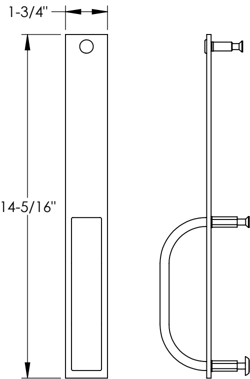
TRIM NO. 810 FLL DESIGN
