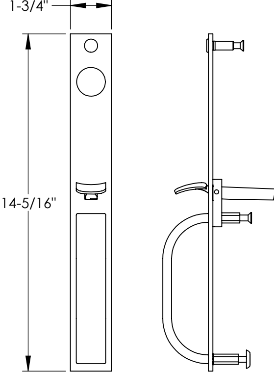
TRIM NO. 866 FLL DESIGN
