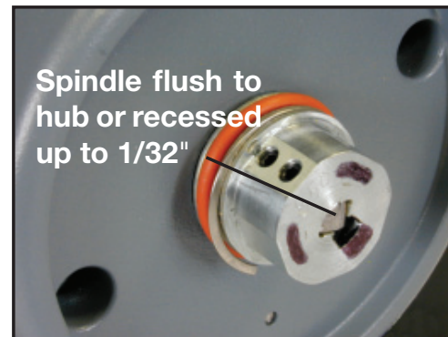
Figure 22 - Spindle Flush or Recessed
