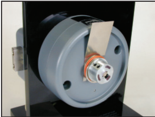
Figure 24 - Place Gauge Between Dial Hub & Bushing
