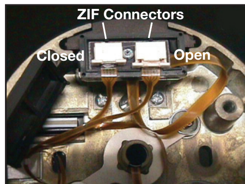
Figure 13 - Closed & Open ZIF Connectors
