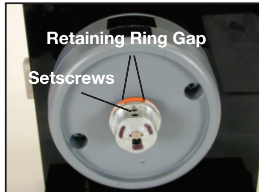
Figure 29 - Align Retaining Ring
