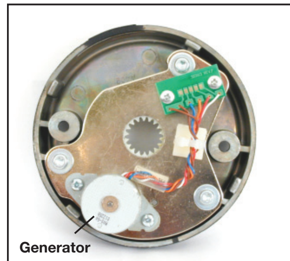
Figure 17 - Dial Ring Cover
