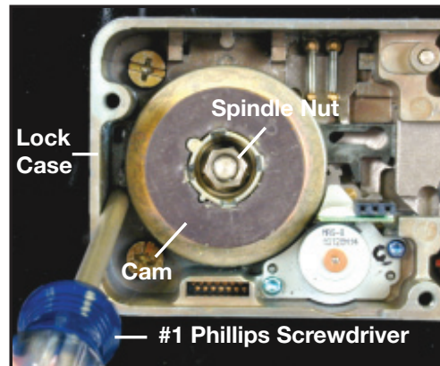
Figure 20 - Secure Drive Cam
