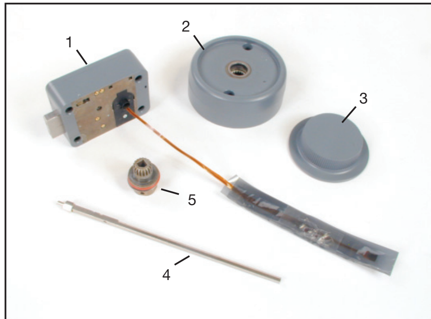
Figure 1 - X-09 Lock Parts
