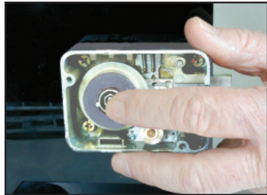
Figure 25 - Maintain Pressure on Spindle Assembly
