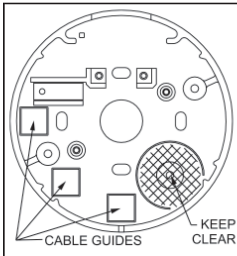
Figure 16 - Cable Guide Locators
