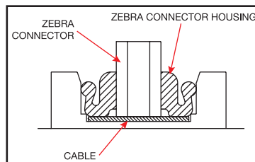
Figure 14 - Zebra Assembly
