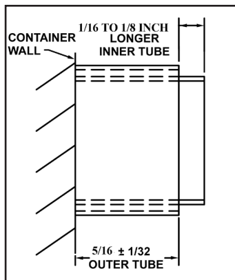
Figure 9 - Inner and Outer Tubes
