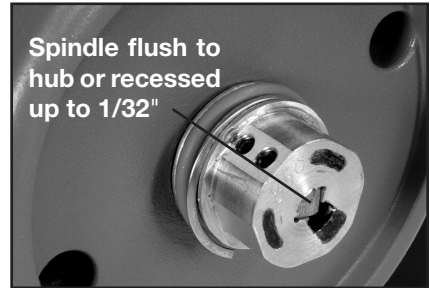
Figure 18 - Spindle Flush or Recessed
