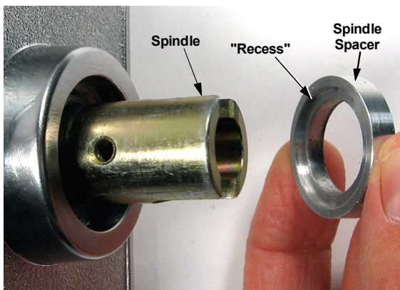
Spindle Spacer MUST be placed with "Recess" facing the spindle
