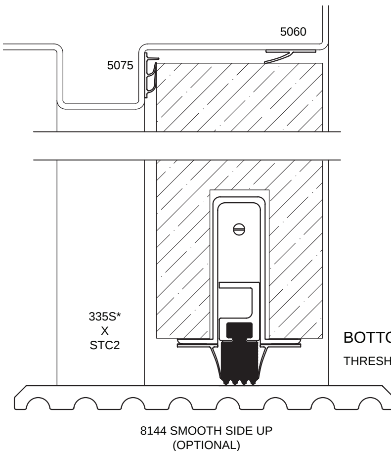
TOP OF FRAME HEADER / JAMB AND DOOR
