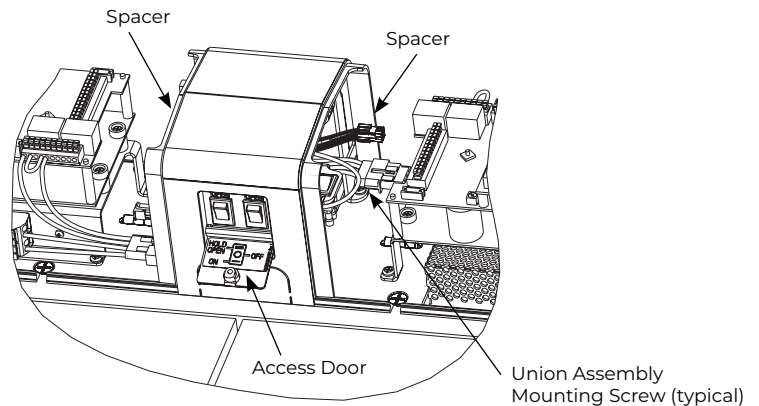
Figure 18 Union Assembly - View From Floor
