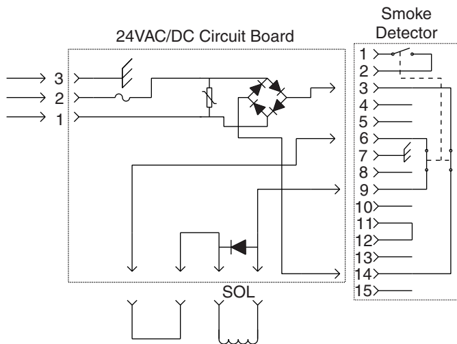
Primary Unit Single Station Wiring Diagram (24VAC/DC Input)
