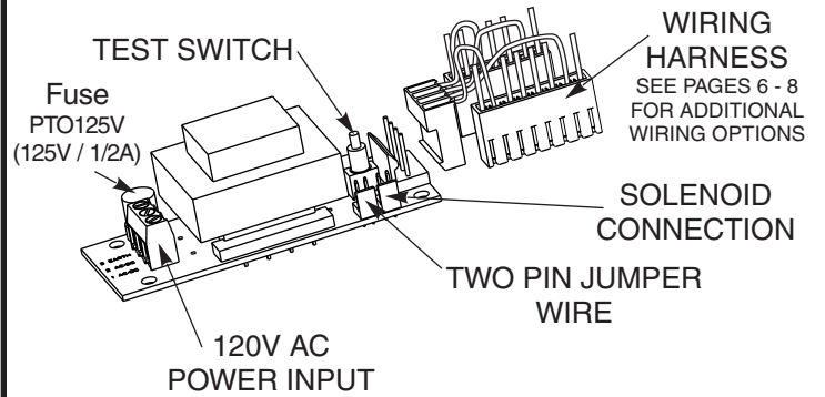
Support Unit Single Station Wiring Diagram (120VAC Input)
