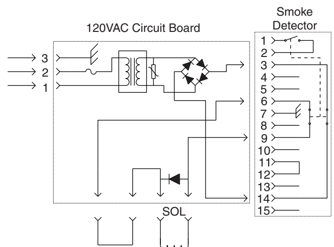
Primary Unit Single Station Wiring Diagram (120VAC Input)
