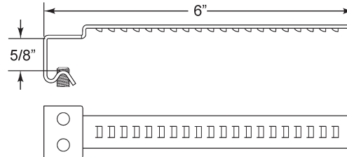
729RS-3 adjustable strap for 3/8" to 5/8" material
